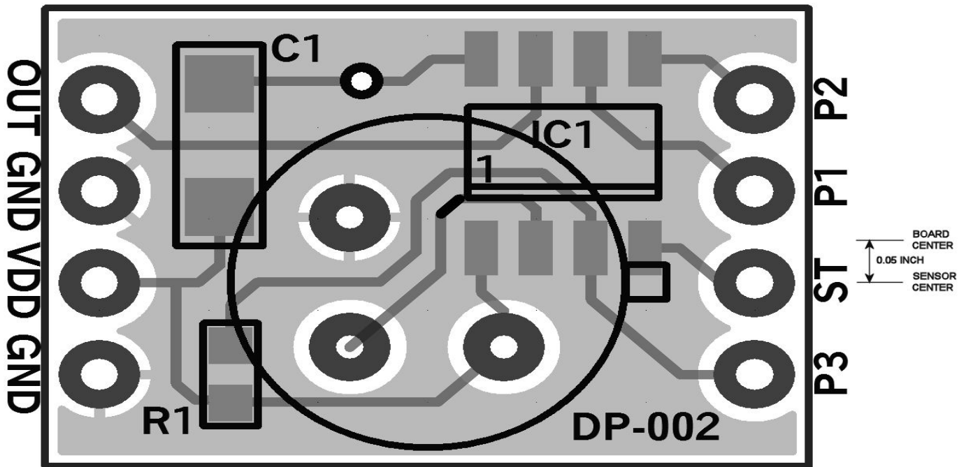
FIGURE 2 COMPONENT SIDE VIEW
