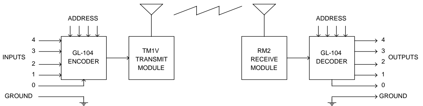
Block diagram of typical wireless remote control
